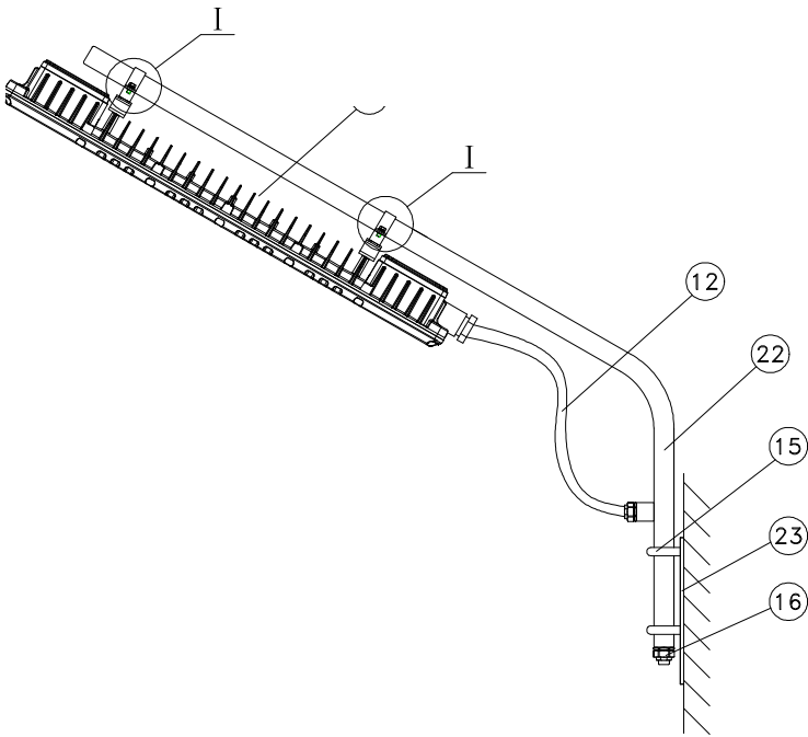
Stanchion(On Wall )
