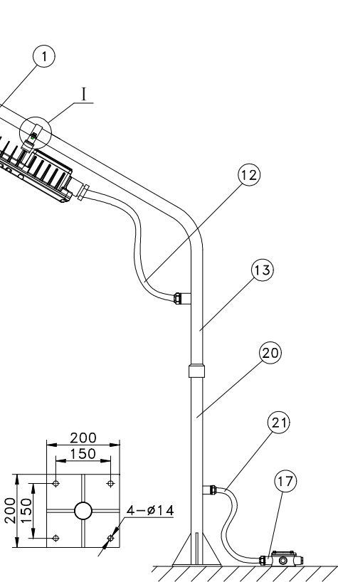
Stanchion(with Flange)
